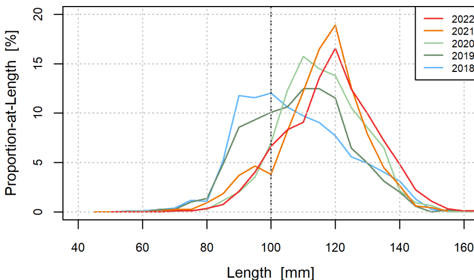
Figure 4.6: Annual population length distributions in 5-mm size bins from annual dredge surveys in Area 27.4.b.S. The vertical dashed line indicates MLS.
